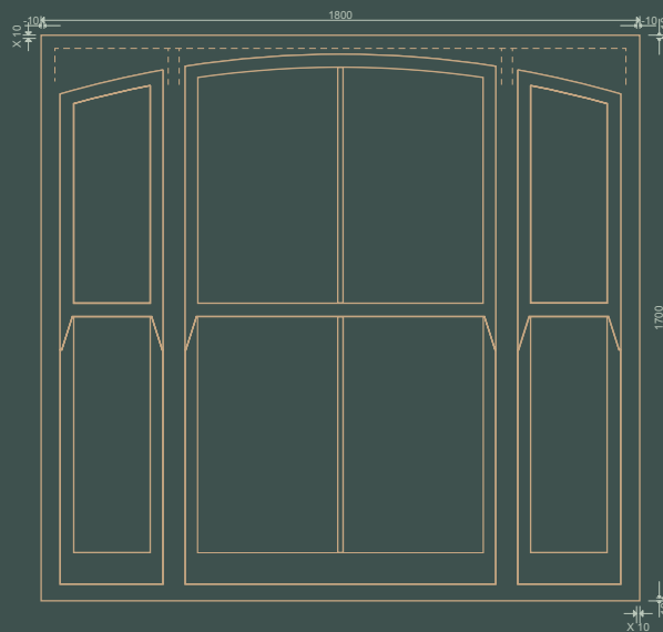
SASH 7
