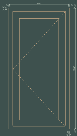
CASEMENT 1
