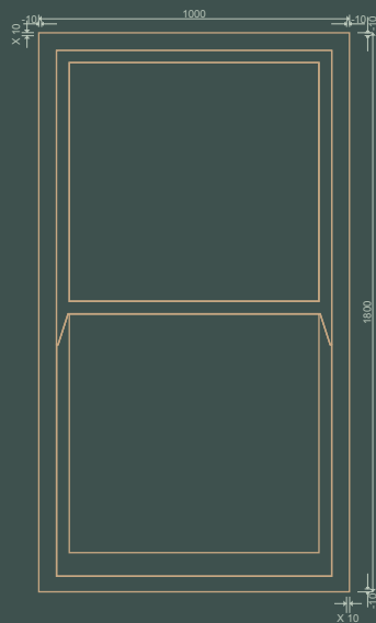
SASH 1
