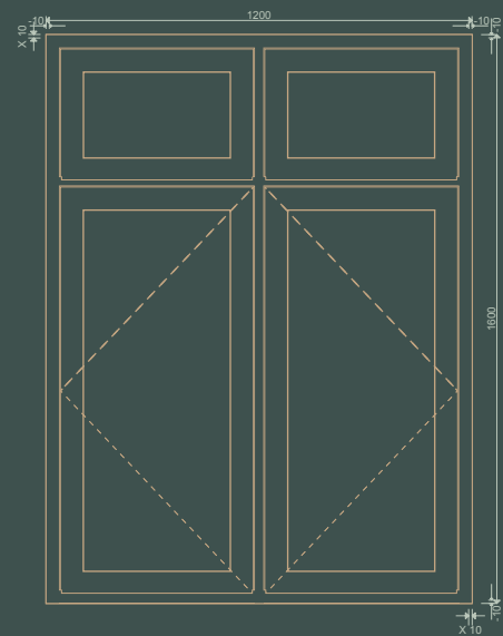
CASEMENT 5
