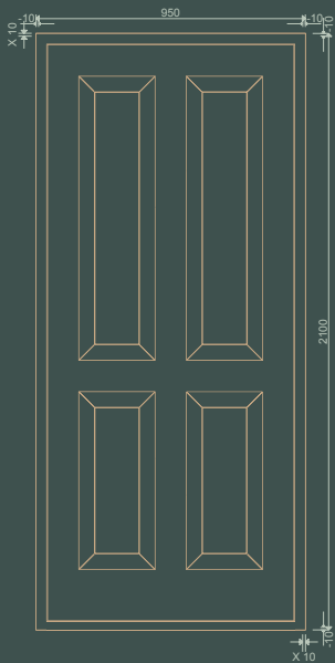
ENTRANCE DOOR 1
