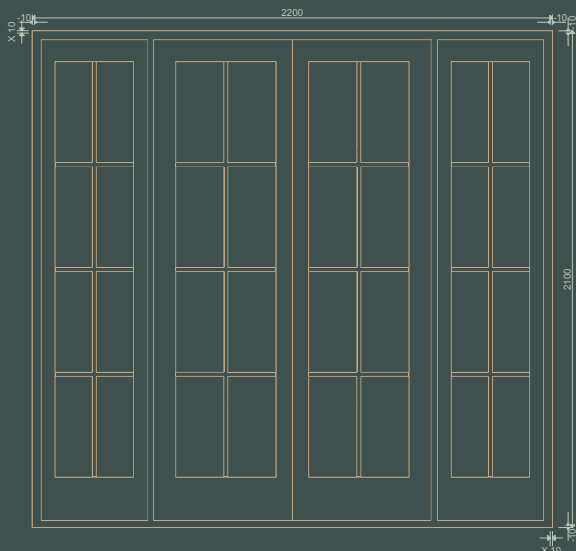
FRENCH DOOR 6
