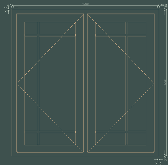
CASEMENT 6
