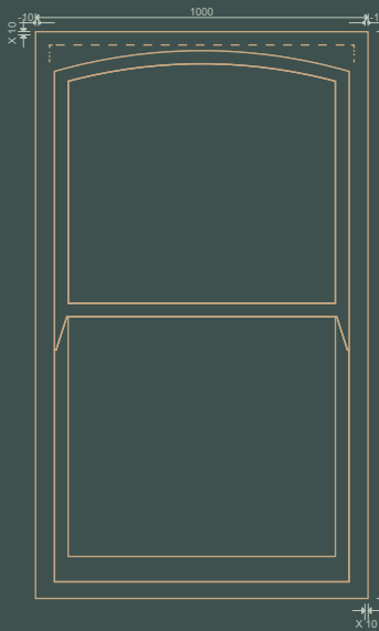
SASH 6
