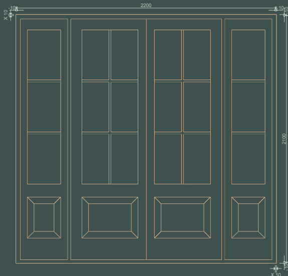
FRENCH DOOR 8
