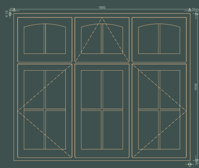
CASEMENT 8
