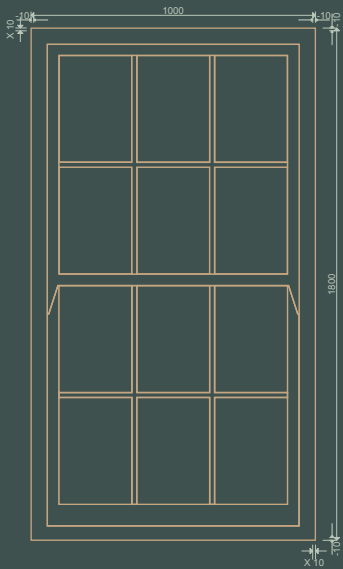
SASH 4
