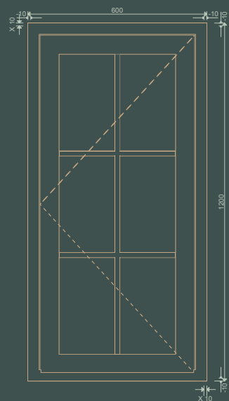
CASEMENT 2
