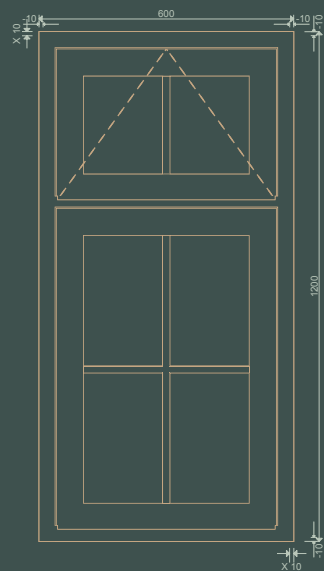
CASEMENT 4
