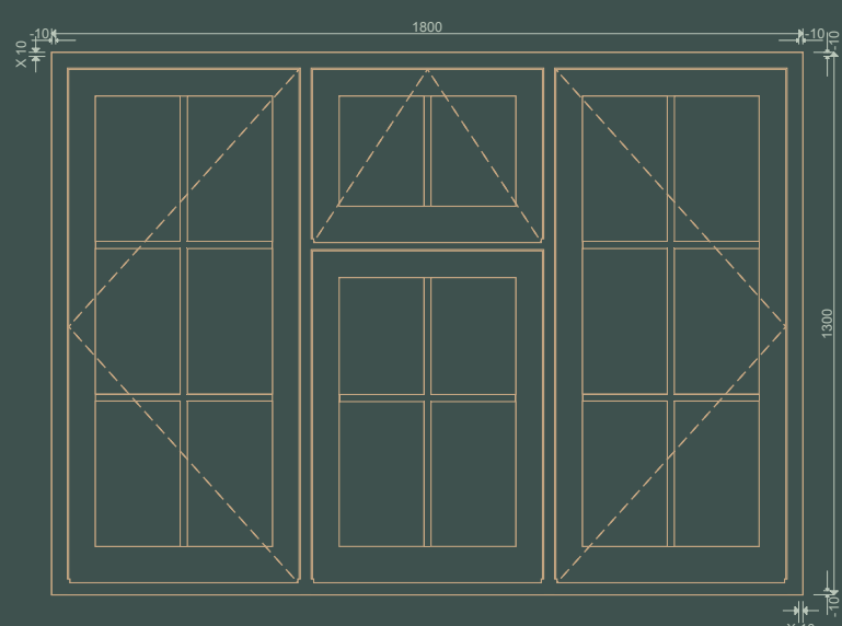
CASEMENT 7
