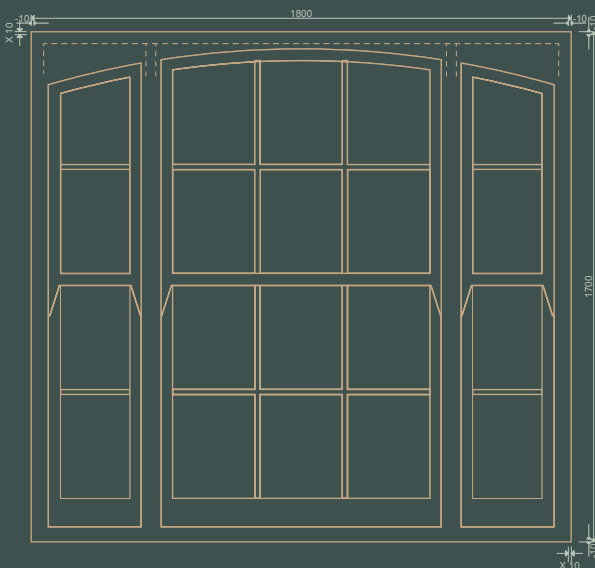
SASH 8
