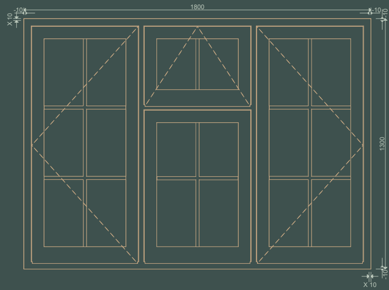
CASEMENT 7
