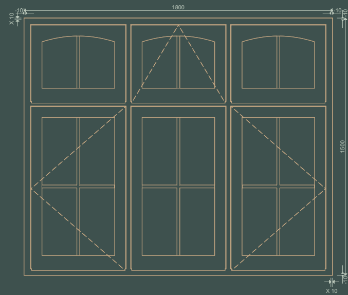
CASEMENT 8
