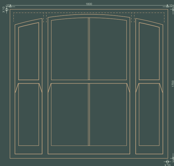
SASH 7
