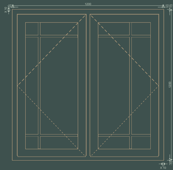
CASEMENT 6
